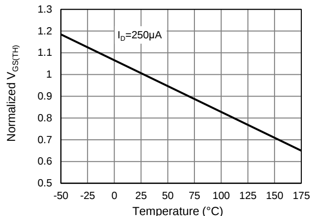
Figure 8: Threshold Voltage vs. Junction Temperature
