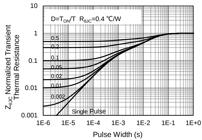
Figure 14: Normalized Maximum Transient Thermal Impedance
