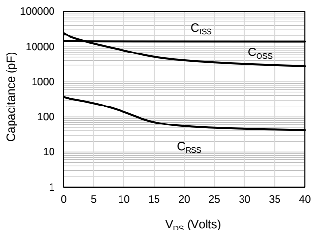
Figure 10: Capacitance Characteristics
