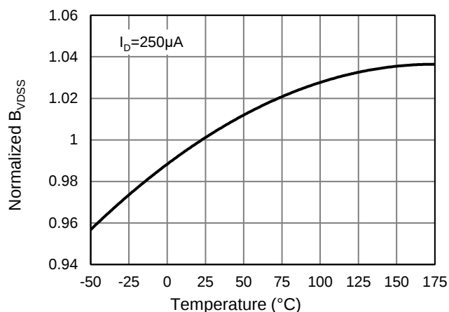
Figure 7: Breakdown Voltage vs. Junction Temperature
