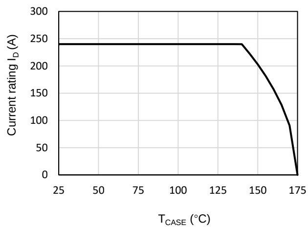
Figure 12: Current De-rating
