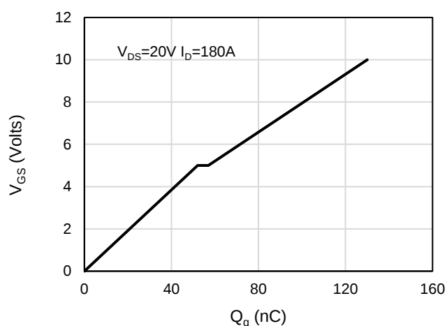
Figure 9: Gate-Charge Characteristics
