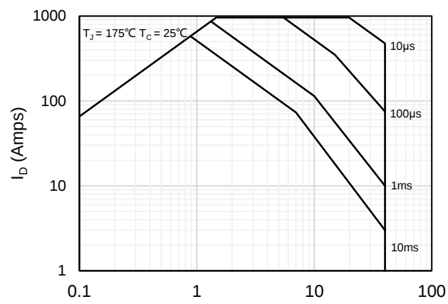
Figure 13: Maximum Forward Biased Safe Operating Area
